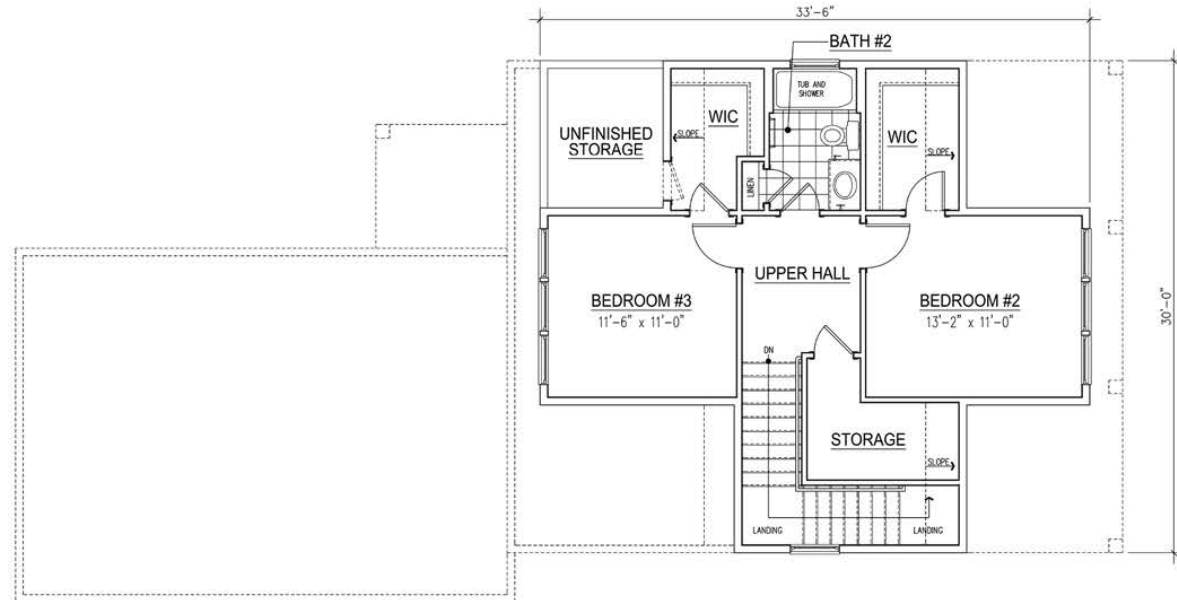
SECOND FLOOR
