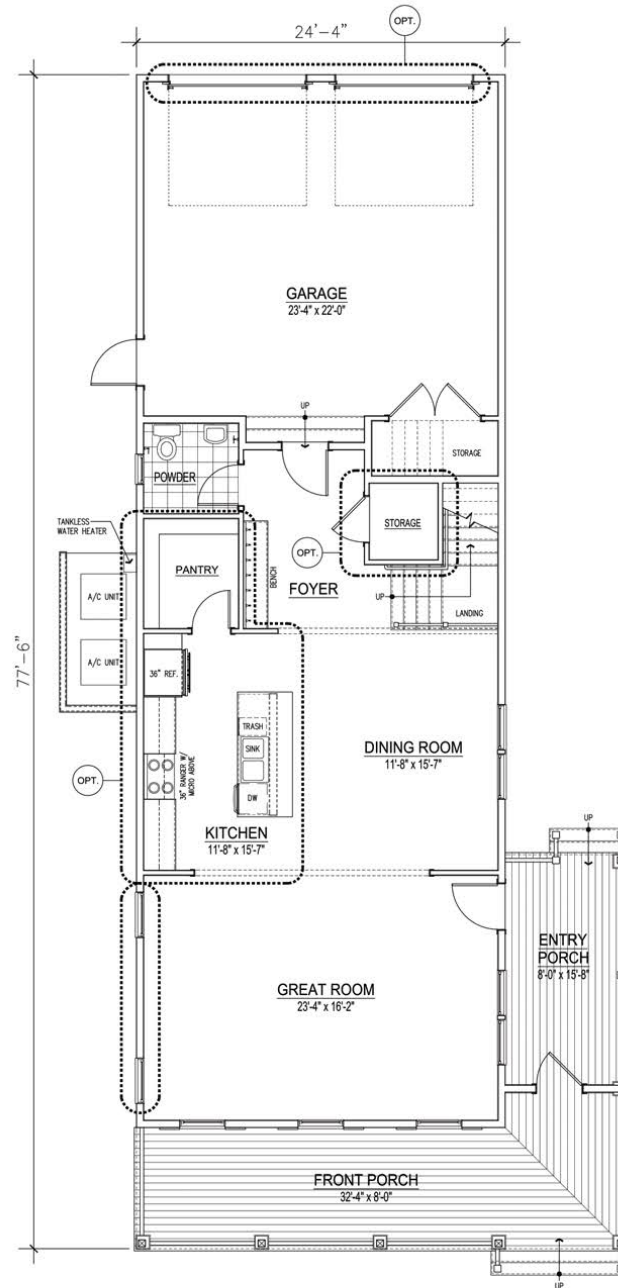
FIRST FLOOR
