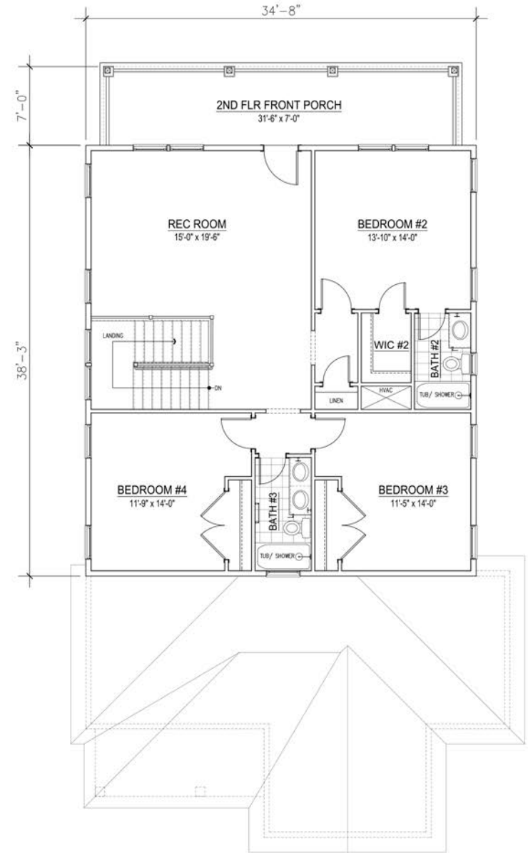
SECOND FLOOR
