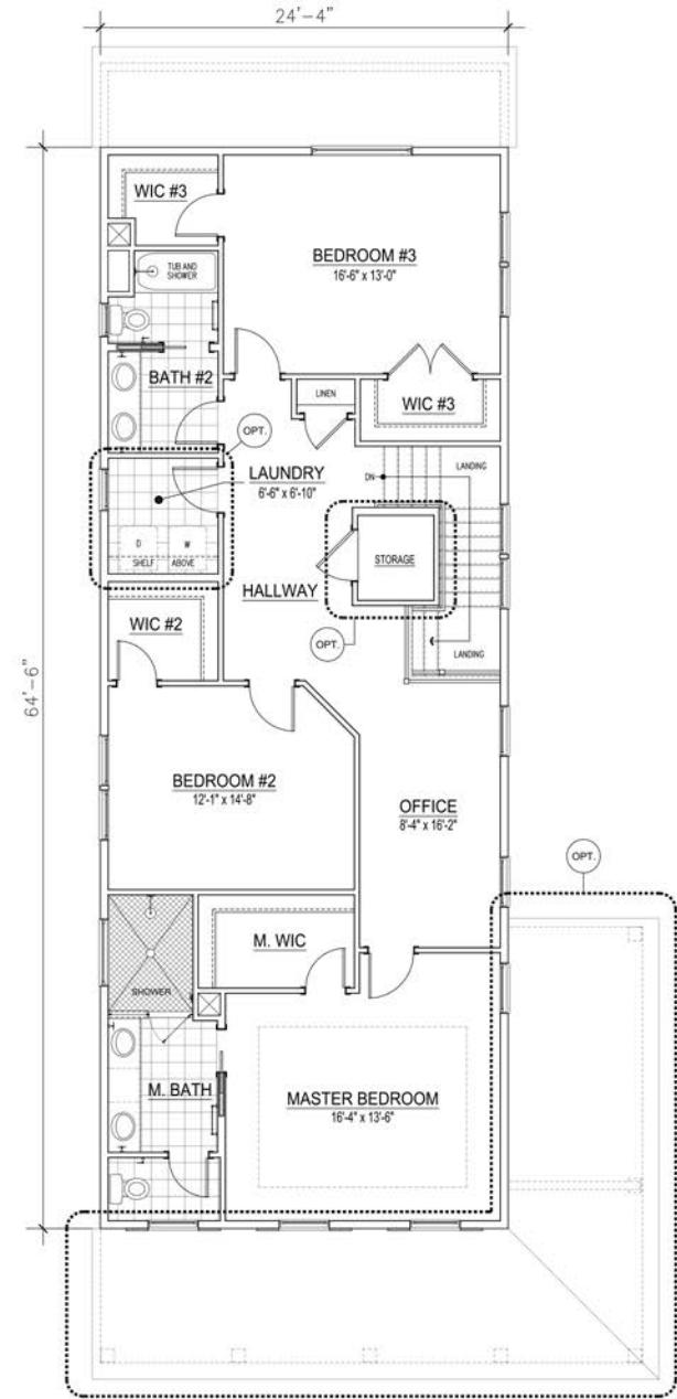
SECOND FLOOR
